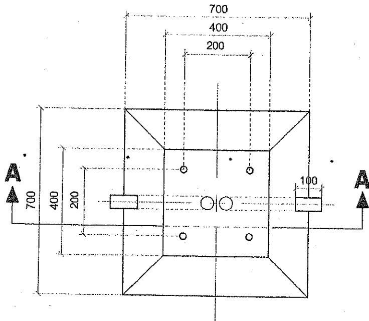
PLAN SCALE
