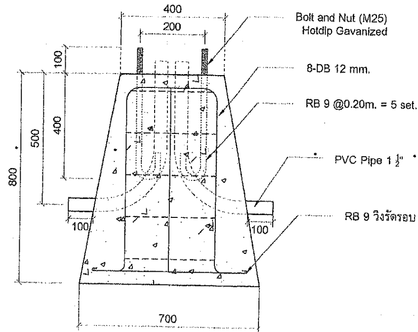
SECTION A - A SCALE
