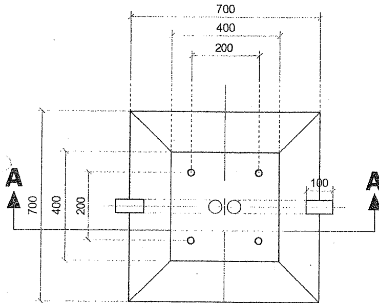
PLAN SCALE -
